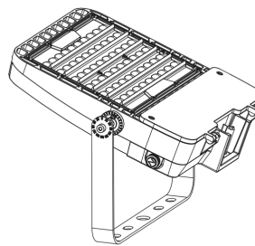
(Trunnion)
